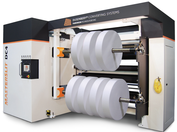
DC4 Center Slitter Rewinder
